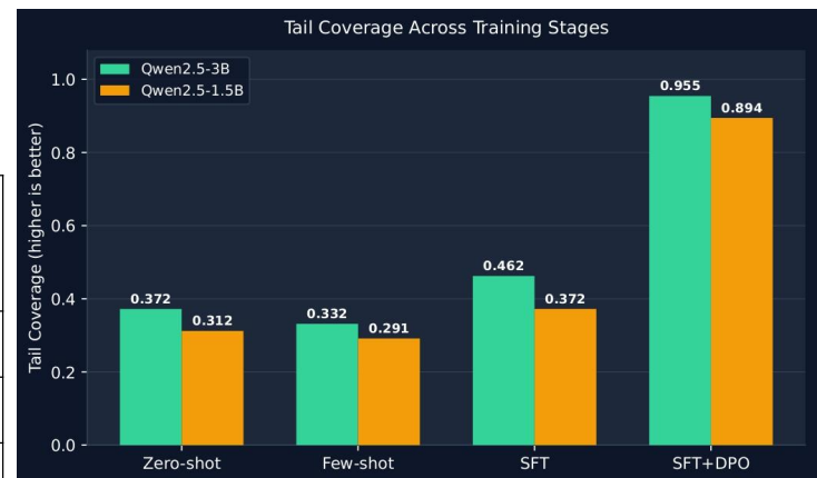
Figure 3: Tail Coverage (TailCov) across training stages. Higher is better. SFT+DPO dramatically improves tail coverage, especially for the 3B model.
