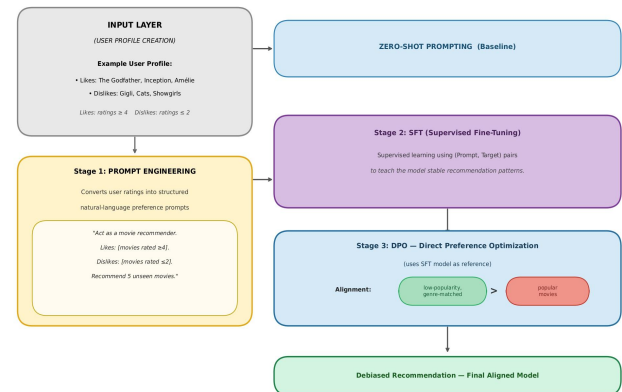
Figure 1: End-to-end pipeline: MovieLens-100K data flows through zero-shot/few-shot prompting, popularity-capped SFT, and DPO preference alignment, evaluated on ARP and TailCov.
