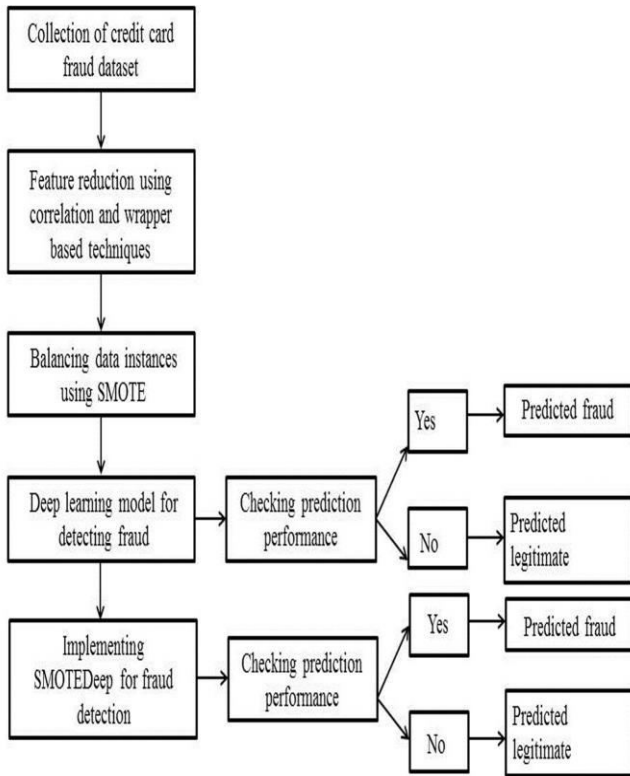
Fig1. The pipeline of credit card fraud detection
