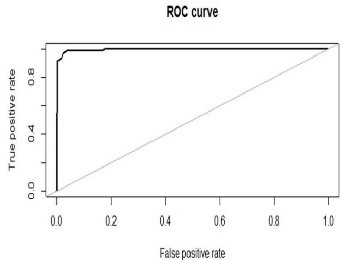
Fig 4. The performance of SMOTEDeep shown in ROC curve indicating its predictive performance
